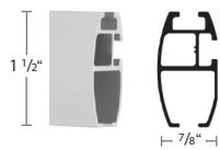
DJB8084020-XX 1 1/2" Oval Rail Stock Length: 19.7'
